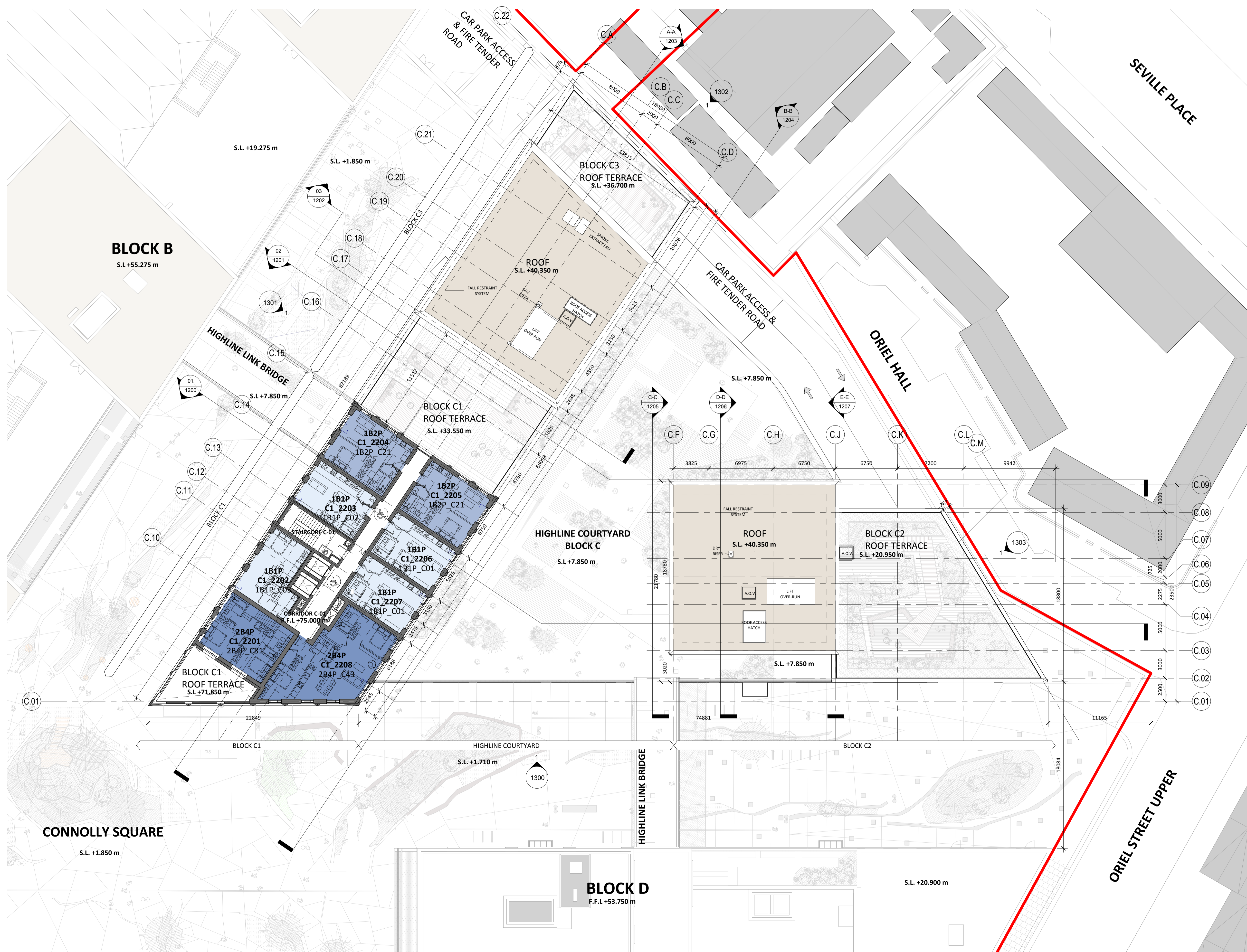
1 BLOCK C PLAN_LEVEL 22 1 : 200
